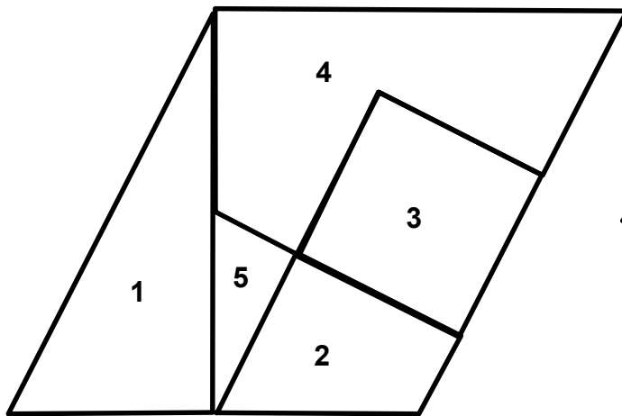
Parallelogram
