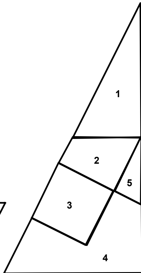
Right-angled Triangle
