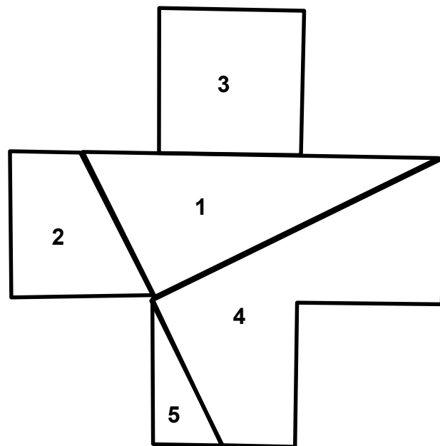
Greek Cross
