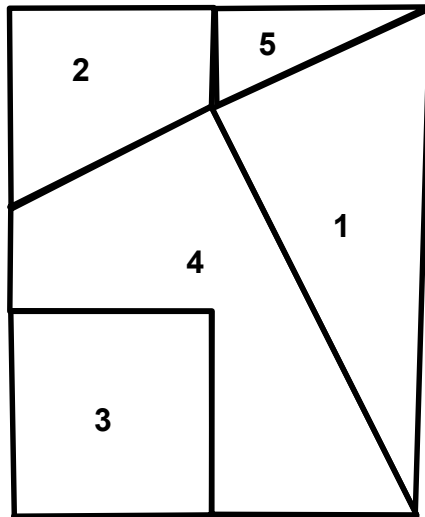
Rectangle
